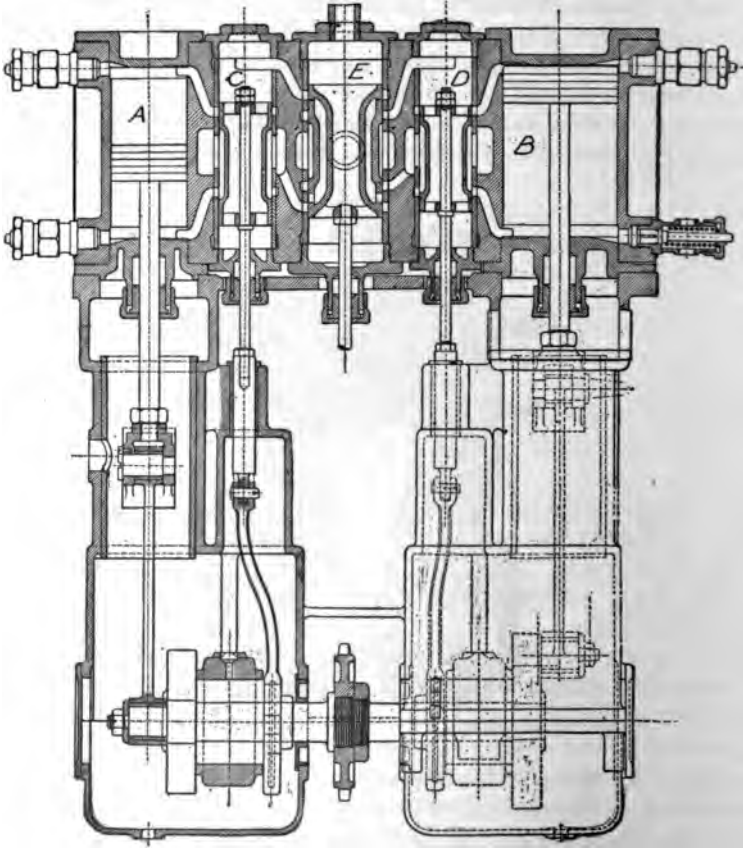
FIG. 376.—Section of the Stearns Compound Steam Carriage Engine. A is the high-pressure cylinder; B , the low-pressure cylinder; C and D , the steam valves operated by single eccentrics; E , the central control valve and chamber.
